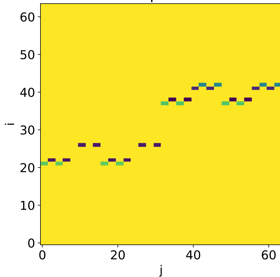
heatmap of cost matrix c_{ij} with n = 4
