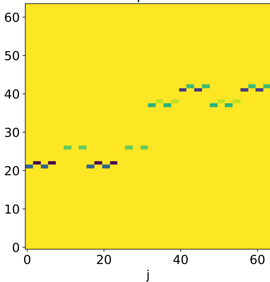
heatmap of cost matrix c_{ij} with n = 4
